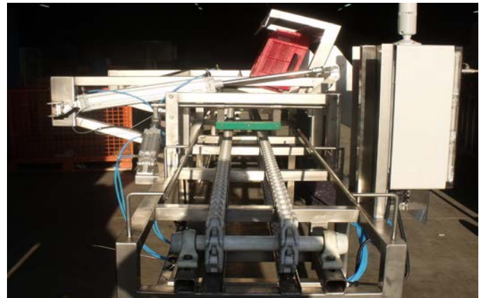
CRATE DUMPER
